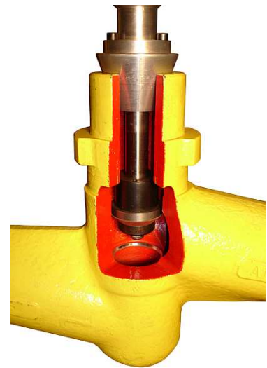
Grinding Device for machining tapered seat valves in connection with the Ventilette machines
