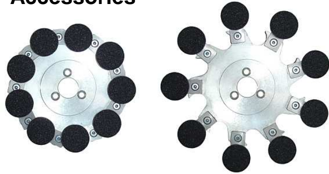
Planet Disc DN 200 mm - Swivel holders with grinding discs at min. (left) and max. (right) external Ø
